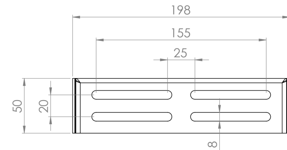
Mount bracket overall dimensions and fixing pattern
